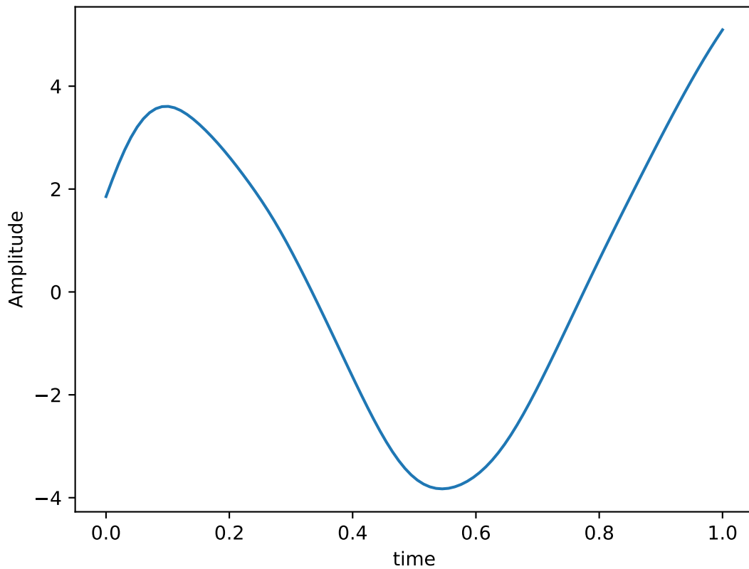
Control Hamiltonian: IZI
