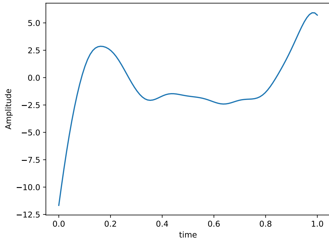
Control Hamiltonian: IY
