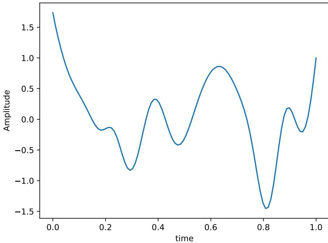
Control Hamiltonian: XII
