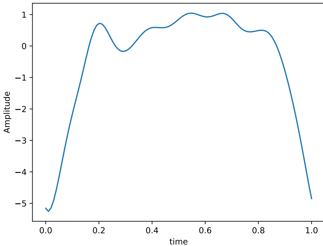
Control Hamiltonian: IXI
