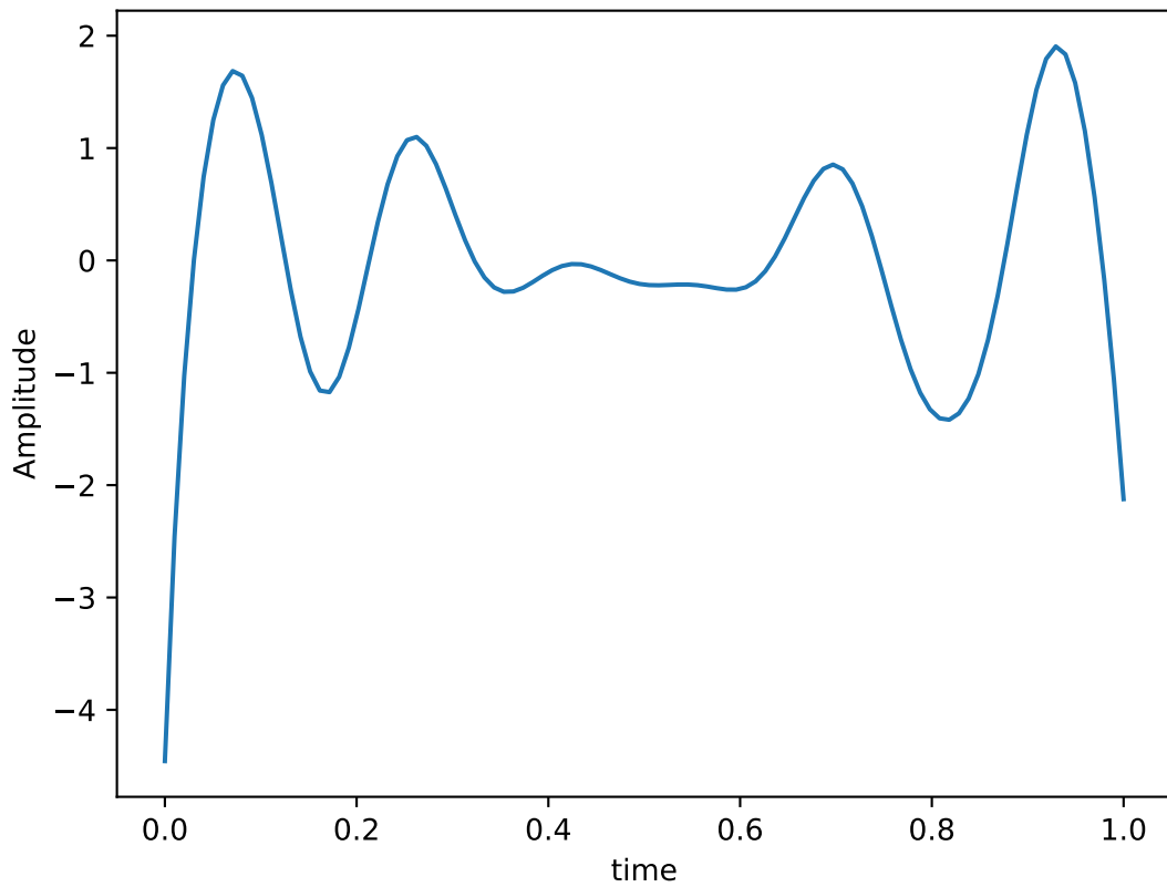
Control Hamiltonian: ZZI
