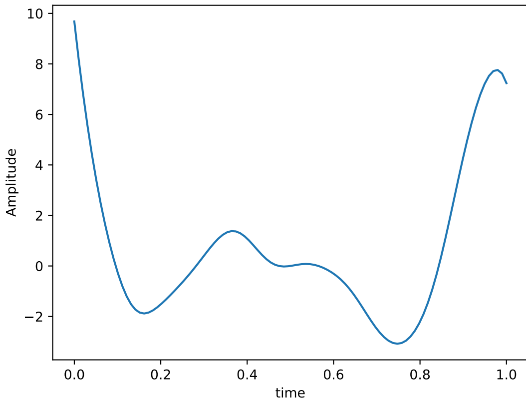
Control Hamiltonian: IIX
