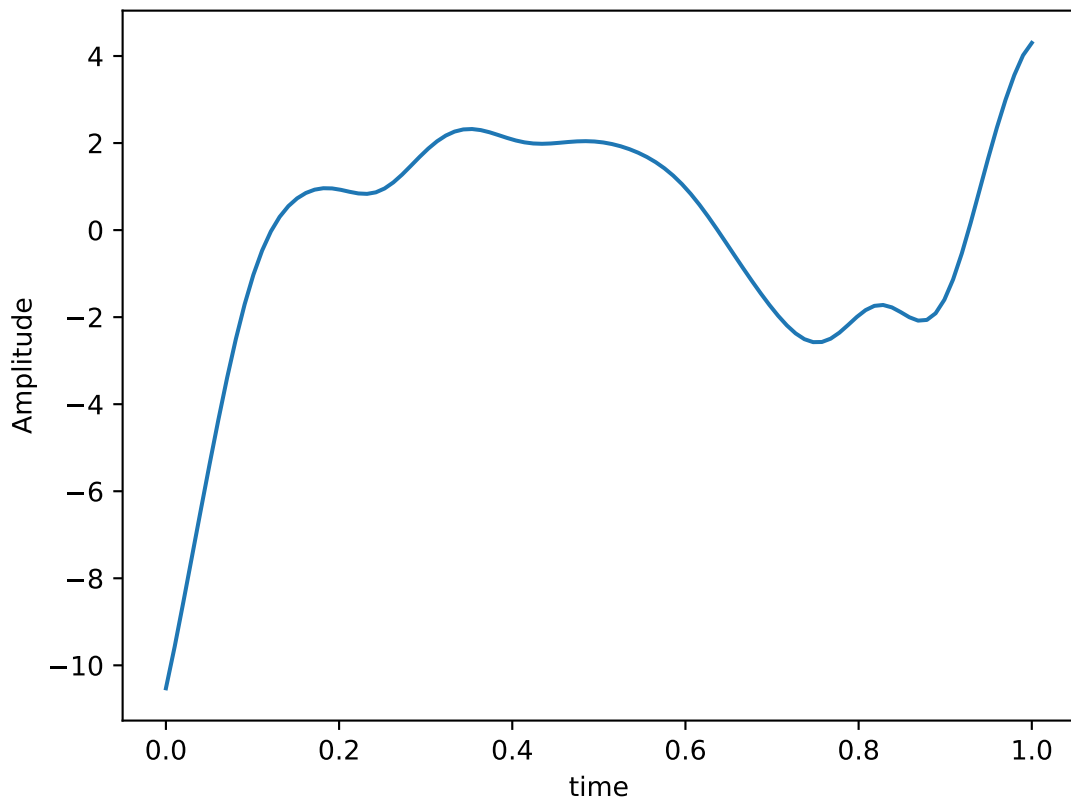
Control Hamiltonian: YII
