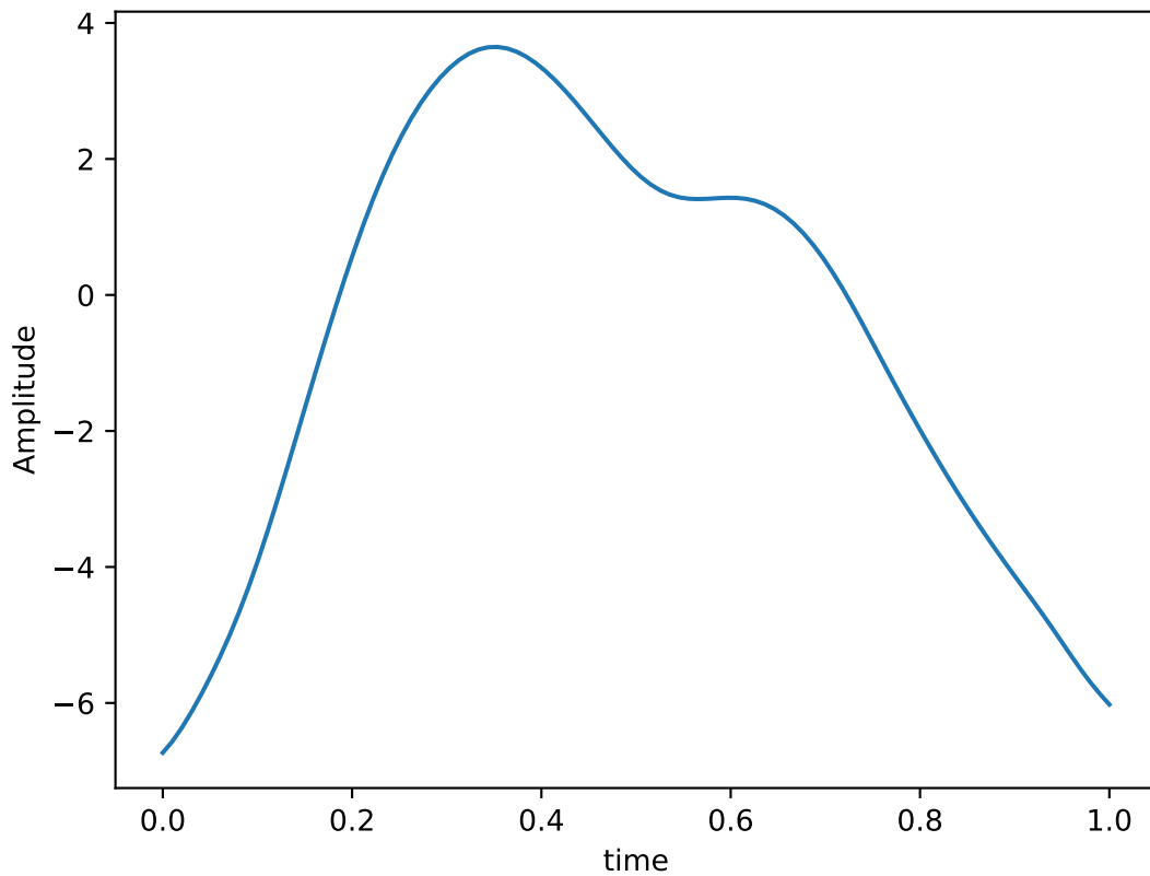
Control Hamiltonian: ZII
