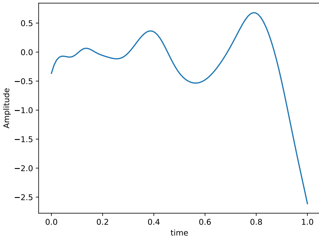
Control Hamiltonian: IIZ
