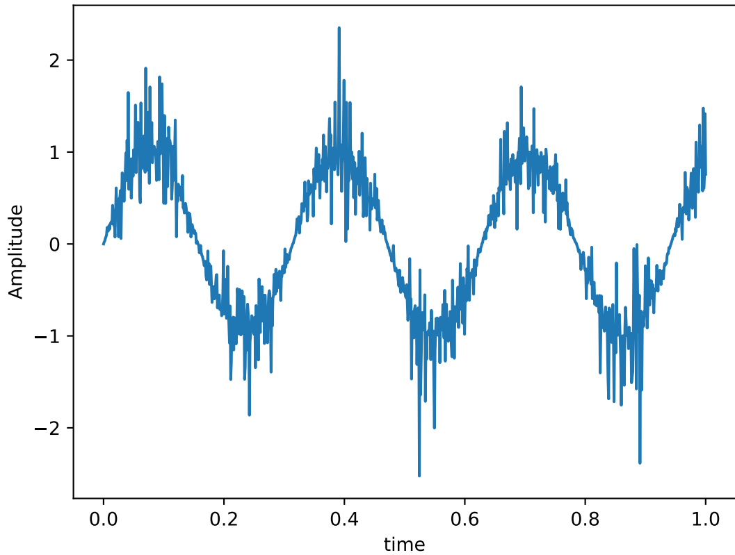
Control Hamiltonian: X
