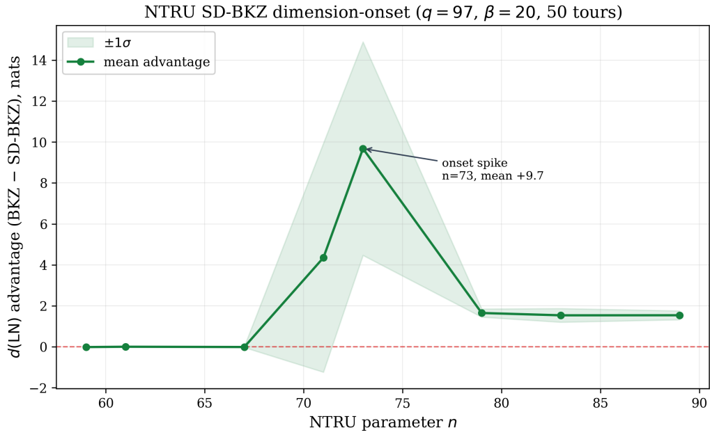
Figure 1: NTRU SD-BKZ dimension-onset ( q = 97, \beta = 20, 50 tours, 20 seeds per n , \pm 1\sigma band; in the bimodal onset zone n = 71 – 73 the band is a spread indicator only, not a distributional summary). The signed advantage is reference-robust at the spike (Section 2.3); shown here for the dimension transition. Recomputed from the per-seed advantage field.
