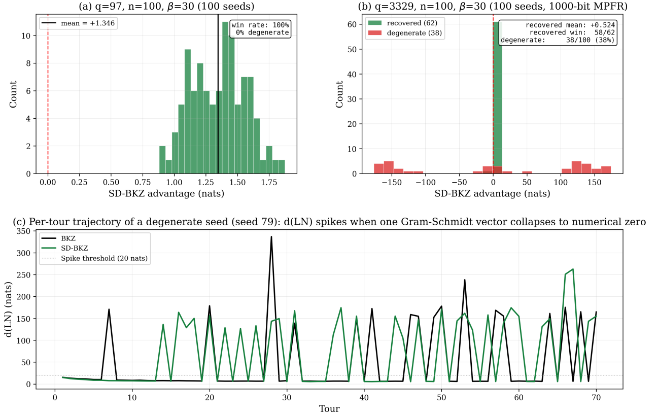
Figure 12. fpLLL Gram-Schmidt cancellation at q = 3329 (ML-KEM modulus), n = 100 , \beta = 30 , 100 seeds at 1000-bit MPFR. (a) For comparison, q = 97 at the same parameters: 100 seeds, mean +1.346 nats, 0% degenerate. (b) q = 3329 : 62 clean seeds (green) cluster near +0.524 nats (93.5% win); 38 degenerate seeds (red/orange) scatter across \pm 170 nats depending on which algorithm happened to end in the collapsed state. Classification: 16 BKZ-only, 13 SD-BKZ-only, 9 both. (c) Per-tour trajectory of a degenerate seed: d(LN) spikes to 140–270 nats whenever one Gram-Schmidt vector collapses, then returns to \sim 5 nats on clean tours. Both algorithms hit the attractor on different tours.
