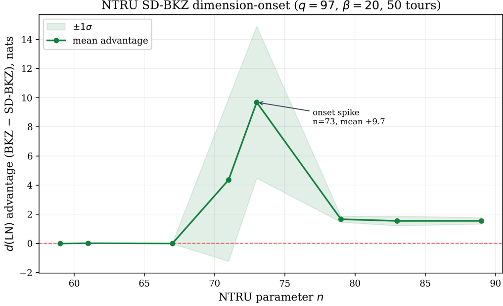
Figure 1: NTRU SD-BKZ dimension-onset ( q = 97 , \beta = 20 , 50 tours, 20 seeds per n , \pm 1\sigma band; in the bimodal onset zone n = 71 – 73 the band is a spread indicator only, not a distributional summary). The signed advantage is reference-robust at the spike (Section 2.3); shown here for the dimension transition. Recomputed from the per-seed advantage field.
