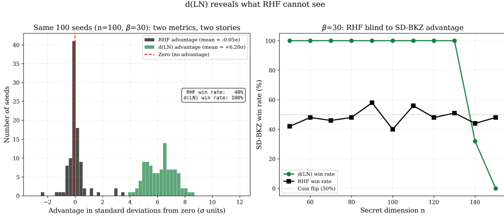
Figure 1: The same 100 seeds ( n=100, \beta=30 ) tell opposite stories depending on the metric. Left: z -score histograms of the per-seed advantage. RHF (grey) is centred on zero (mean -0.05\sigma , coin flip); d(\text{LN}) (green) sits 6.2\sigma from zero with no overlap (this group; peak effect is 9.4\sigma at n=100, \beta=40 ). Right: SD-BKZ win rate by dimension for \beta=30 . d(\text{LN}) shows 100% win rate through n=130 before collapsing; RHF fluctuates around 50% at every dimension, blind to the structural difference.
