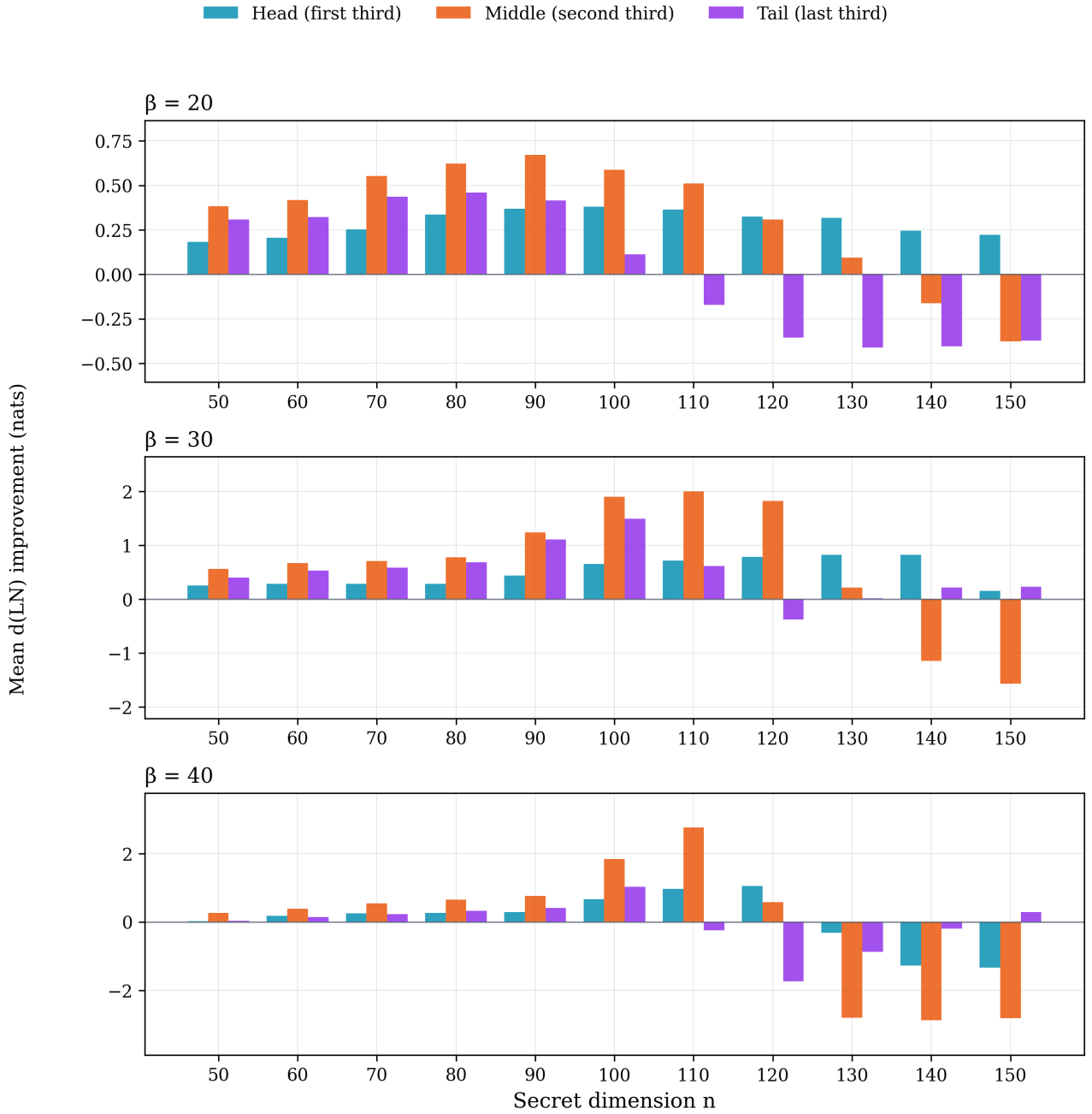
Figure 6. Mean d(\text{LN}) improvement by profile region (head, middle, tail) across all groups, faceted by block size. At \beta = 20 (top), the middle dominates through n = 100 , but the tail flips negative from n = 110 onward as the backward pass loses its reach. At \beta = 30 (middle), the middle peaks at n = 100\text{--}110 (+1.9 to +2.0 nats) before flipping strongly negative at n = 140/150 , indicating BKZ wins the middle at high dimensions. At \beta = 40 (bottom), the cliff is visible: all three regions improve dramatically at n = 100\text{--}110 before collapsing below zero at n \geq 120 , with every region simultaneously flipping sign.
