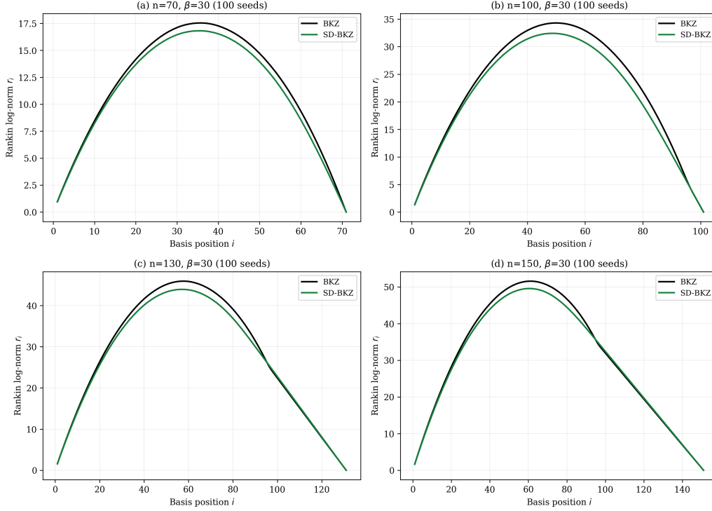
Mean Rankin profile: BKZ vs SD-BKZ ( \beta=30 progression)
