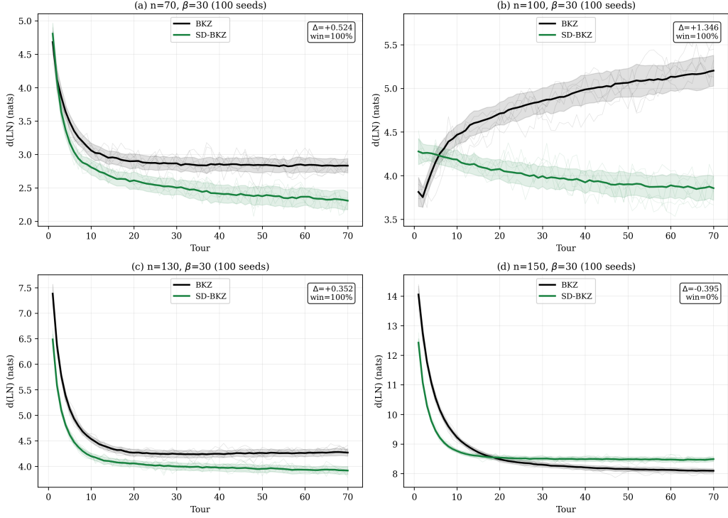
Per-tour convergence: BKZ vs SD-BKZ ( \beta=30 progression)
