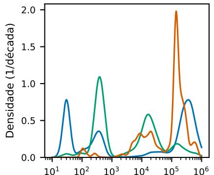
(c) PacketLengthVariance (bytes 2 )
