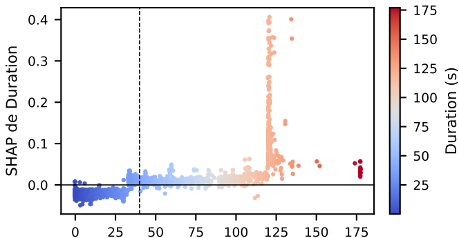
(a) Duration (s)
