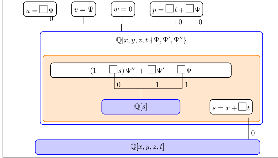
Figure 9: The normalized truncation of Figure 8 used in the computation: a linear ODE in place of the second-degree one, the rotation and scaling freedoms spent, and no mean pressure gradient. Slots fixed by a normalization are written out; the seven remaining boxes carry the nine free constants.
