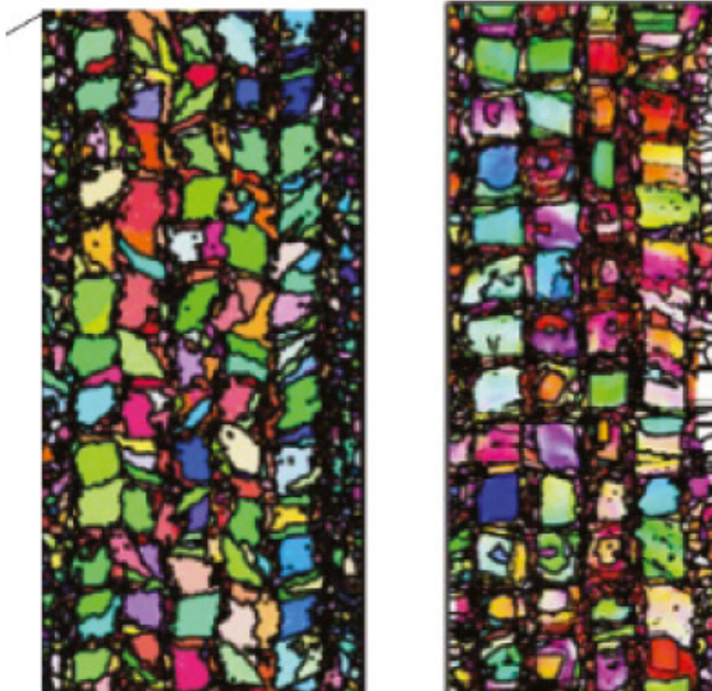
ExaCA CA prediction (left) and AM-Bench EBSD (right). M. Rolchigo et al., Comput. Mater. Sci. 214 (2022) 111692, Fig. 11(b).
