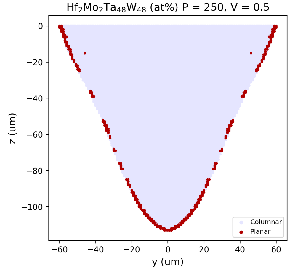
TCAM-derived microstructure classification projected along the solidification front onto a yz slice for the same alloy and process condition.
