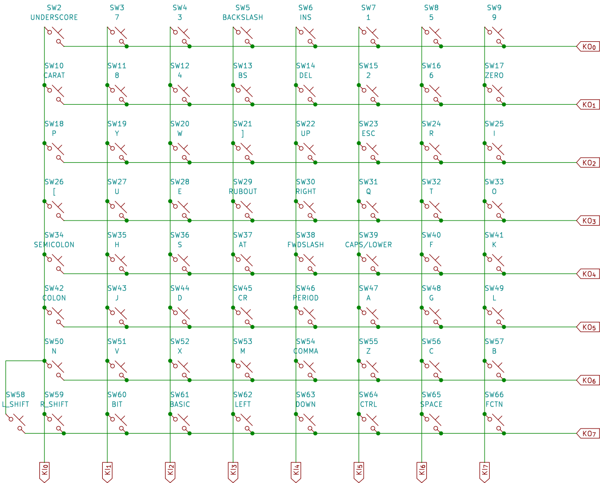
Keyboard Matrix
