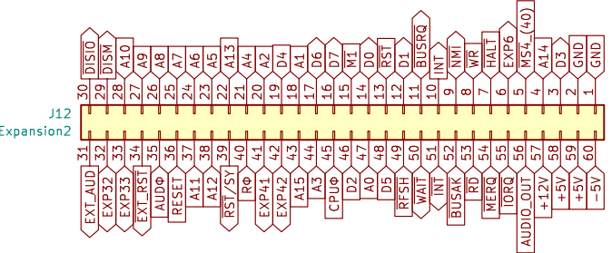
System Expansion (Pen Header) Additional option for connecting/accessing the expansion bus
