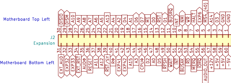
System Expansion (Pen Header) Additional option for connecting/accessing the expansion bus
