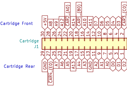
ColecoVision Cartridge
