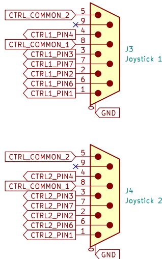
Joysticks Doesn't match ColecoVision as far as I can tell
