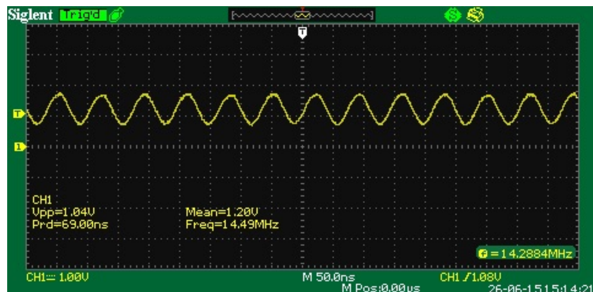
IC16 Pin 3
