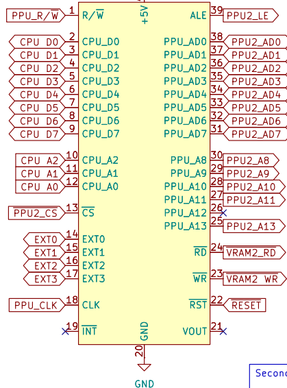
+5V U5B1 RP2C02G PPU #2
