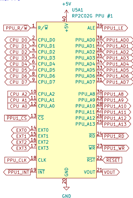
Original PPU
