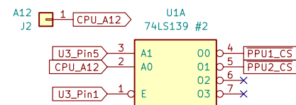
Second 74LS139
