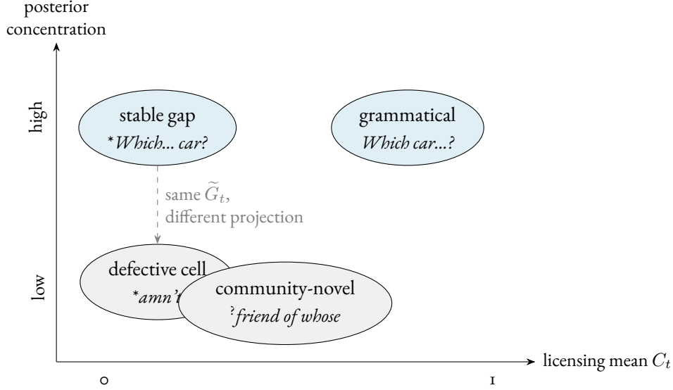
Figure 2: The licensing state has two dimensions, but the mean-product \tilde{G}_t reads only the horizontal one. Stable gaps (dense preemption, posterior concentrated near zero) and defective cells (split candidates, posterior low but diffuse) share a licensing mean and part only on concentration, the axis that predicts satiation, framing sensitivity, and actuation.
