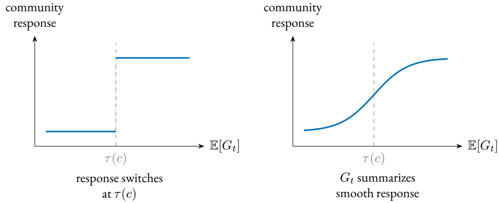
Figure 6: The decision-layer discontinuity check. If asymmetric losses induce a response switch, community treatment of a form should change discontinuously as \mathbb{E}[G_t] crosses the situational threshold \tau(c) (left); if the read-out tracks the posterior mean continuously, treatment should vary smoothly through it (right). A regression-discontinuity design on multinomial hearer responses targets this decision layer, not the constitutive status state itself.
