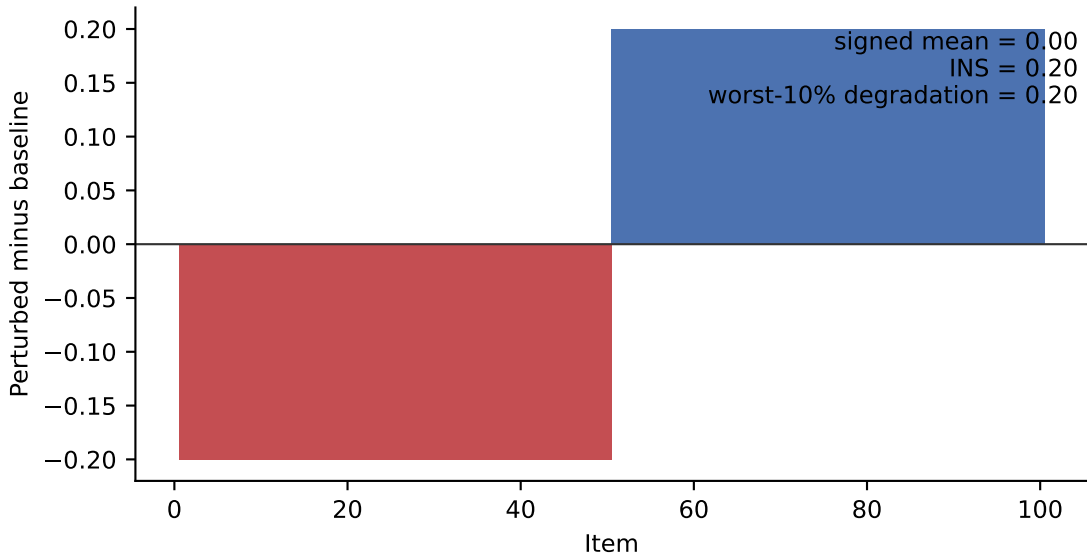
Mean change cancels while item-level instability remains
