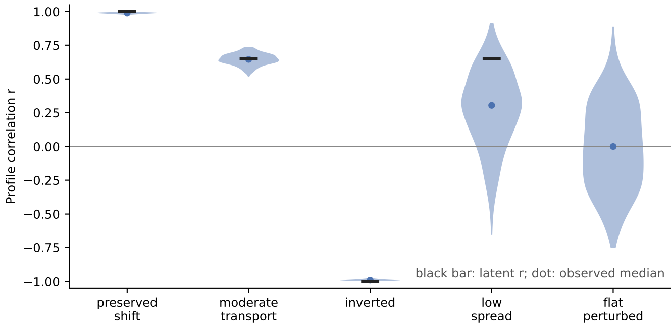
Profile-correlation uncertainty with only ten domain means
