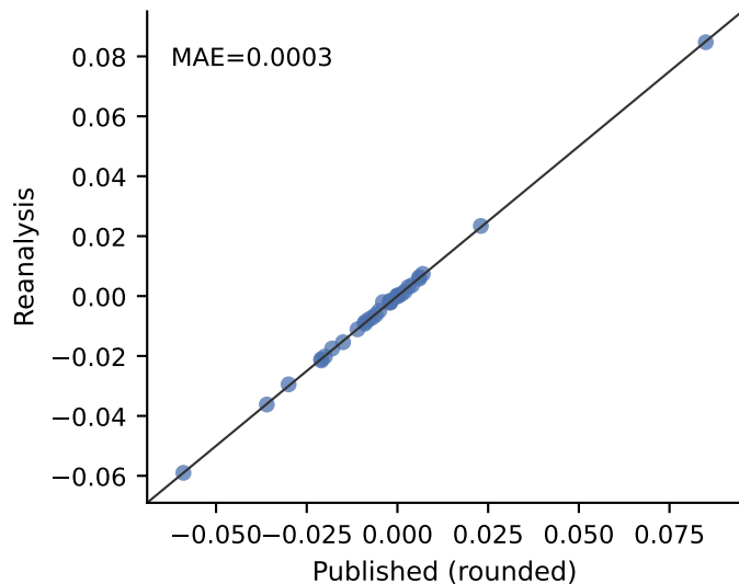
Pseudo-null-adjusted WTD
