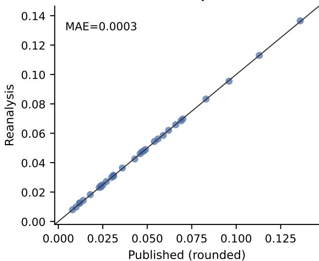
Pseudo-null-adjusted INS
