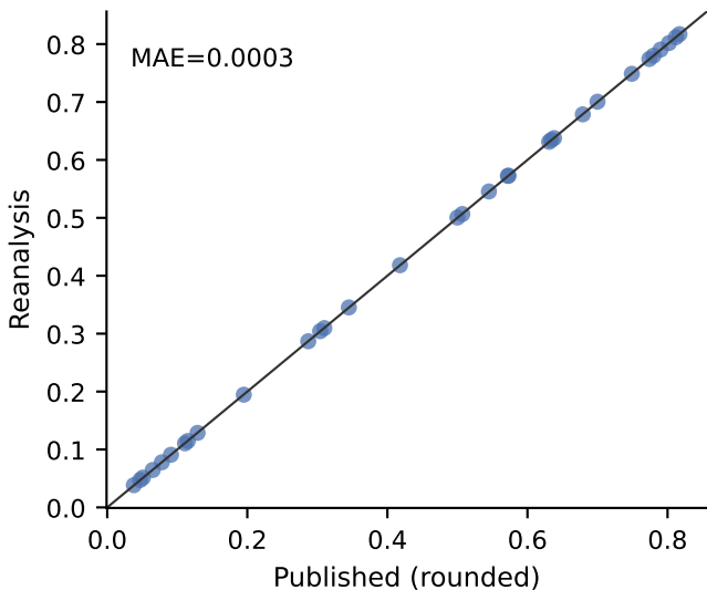
Pseudo-null-adjusted INS
