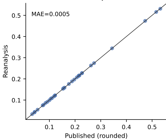
Pseudo-null-adjusted WTD
