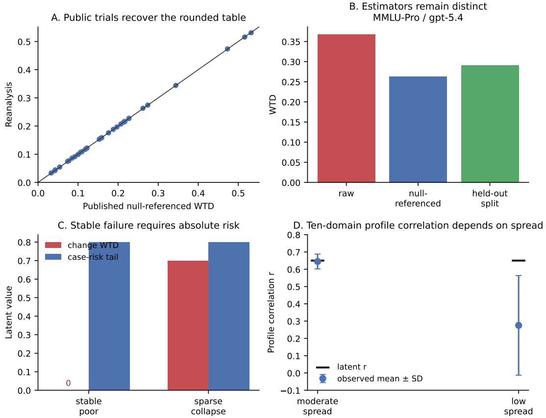
Figure 1: Released-output reproduction and simulation checks. (A) Recomputed null-referenced WTD for all 32 comparisons against the rounded values reported by Zhang et al. (2026, p. 4). (B) Raw, null-referenced, and response-half split WTD for MMLU-Pro-gpt-5.4; the latter two estimate different quantities. (C) A simulation with stable, persistently poor performance on the same items has zero latent WTD but .80 worst-decile latent itemwise expected loss (case-risk WTL). (D) With ten domains and latent r = .65 , correlation estimation remains accurate at moderate profile spread but attenuates under low spread. Full settings and numerical outputs are in the empirical companion.
