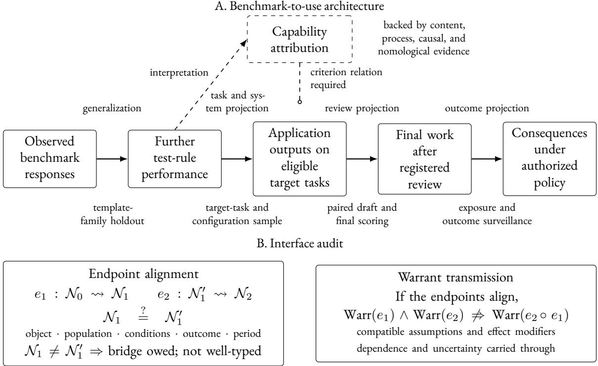
Figure 1: Architecture and interface failures in a benchmark-to-use argument. Panel A matches evidence to projections between empirical endpoints. A capability attribution can be supported while leaving the target cases and criterion relation needed for application performance untested. Panel B distinguishes endpoint mismatch, which leaves the composition ill-typed without a bridge, from failure of warrant transmission across aligned endpoints.
