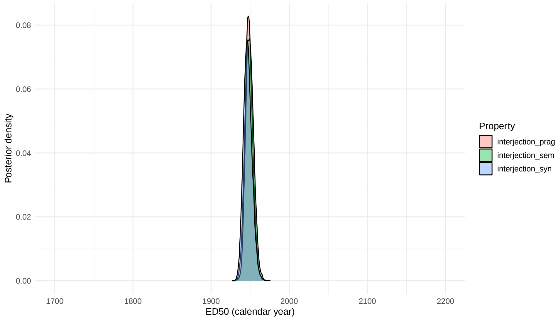
Posterior distributions of ED50 (tau) for each property
