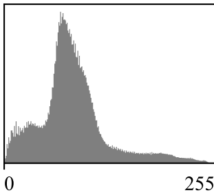
d) CLAHE
