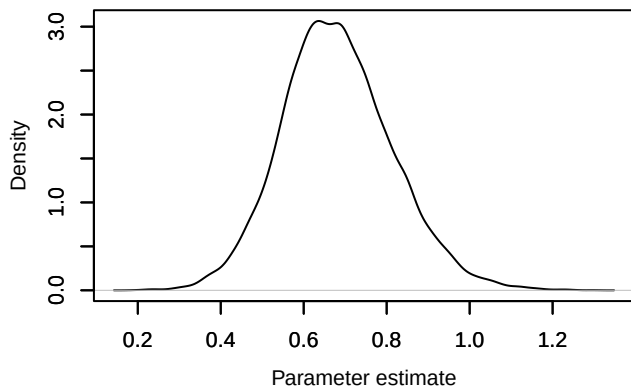
Density – delta[2]
