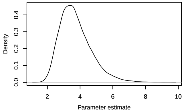
Density – tau_eps[1]
