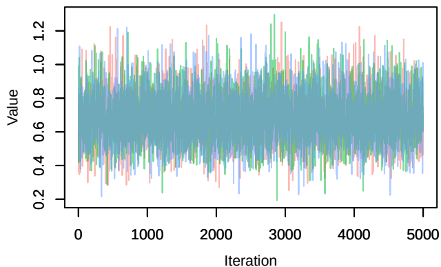
Trace – delta[2]
