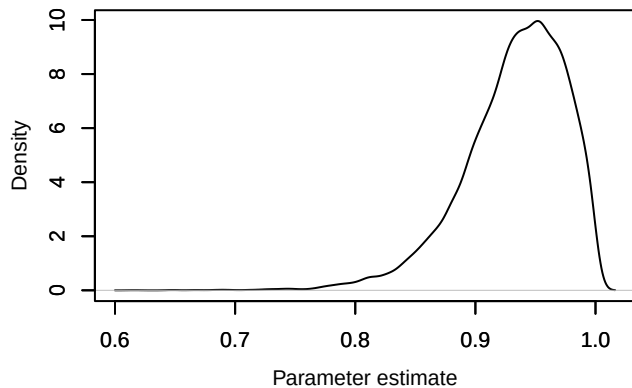
Density – theta[1]
