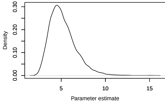
Density – tau_eps[1]
