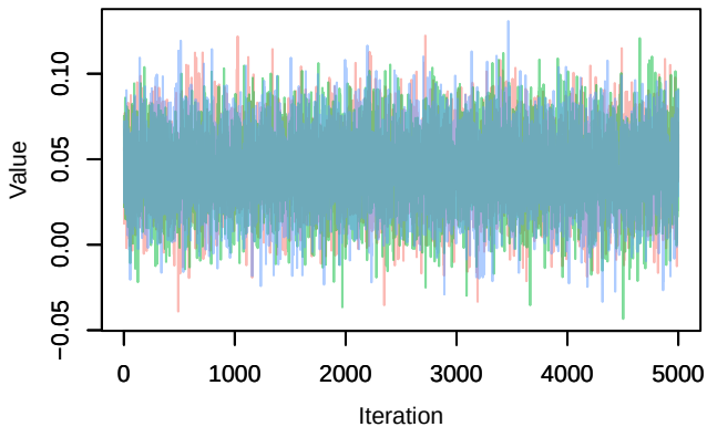
Trace – delta[1]
