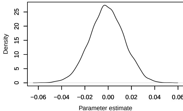
Density – gamma1[1]
