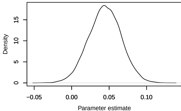
Density – delta[1]
