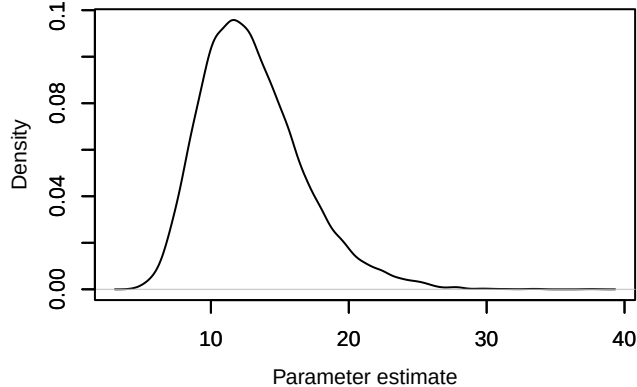
Density – tau_eps[2]
