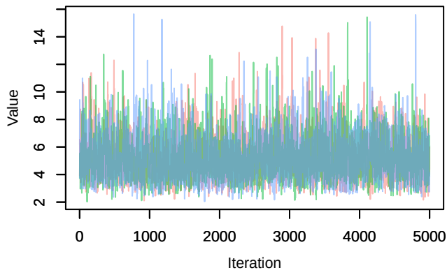
Trace – tau_eps[1]
