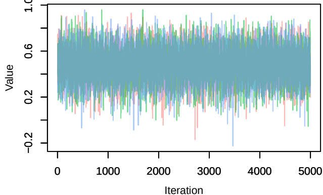
Trace – gamma1[1]
