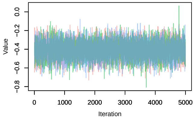
Trace – gamma0[2]
