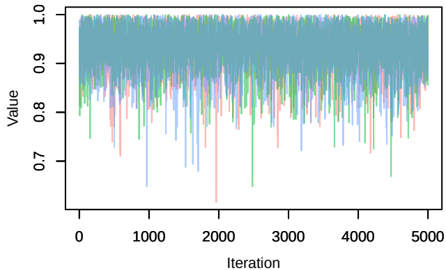
Trace – theta[1]
