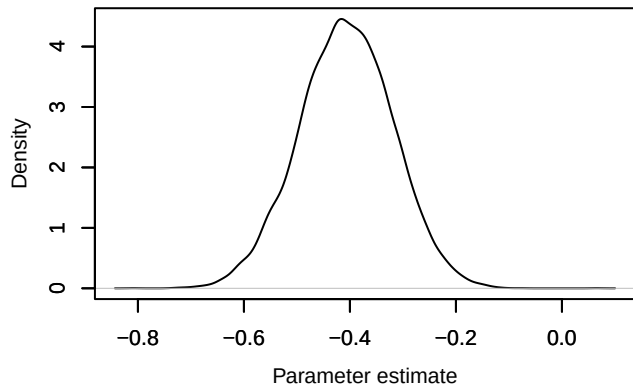
Density – gamma0[2]
