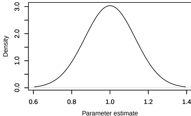
Density – delta[2]
