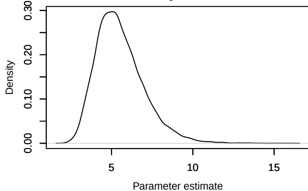
Density – tau_u
