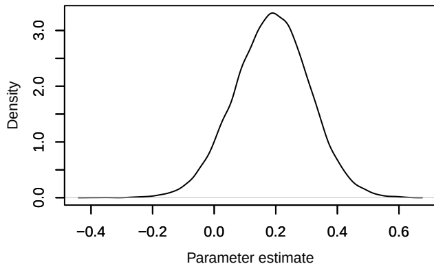
Density – gamma0[2]
