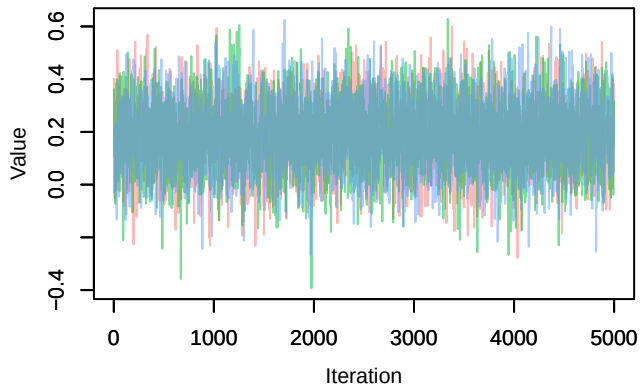
Trace – gamma0[2]
