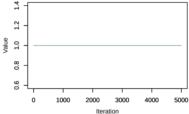
Trace – delta[2]
