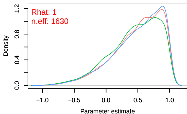
Density – phi[1]
