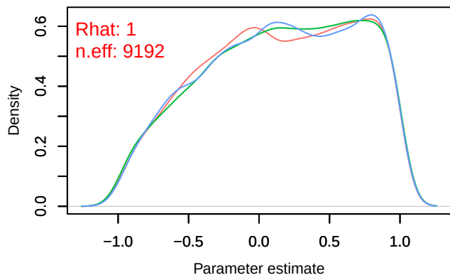
Density – phi[2]
