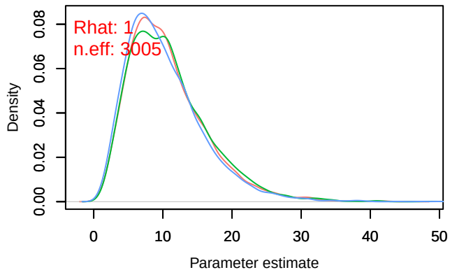
Density – tau_eps[2]
