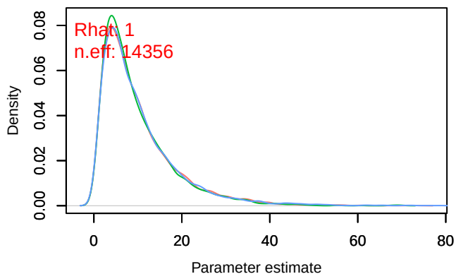
Density – tau_eps[2]
