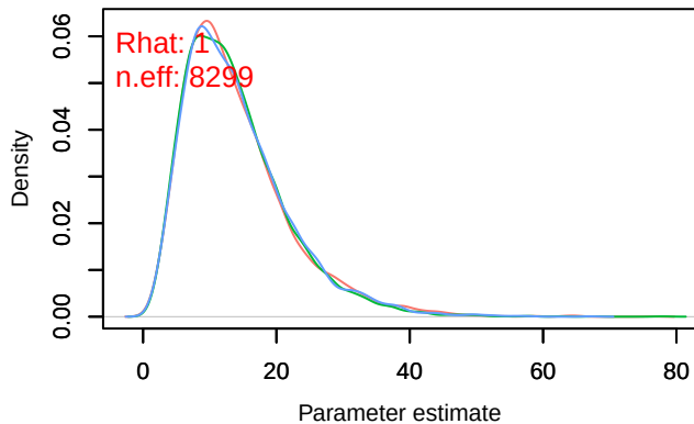
Density – tau_eps[2]
