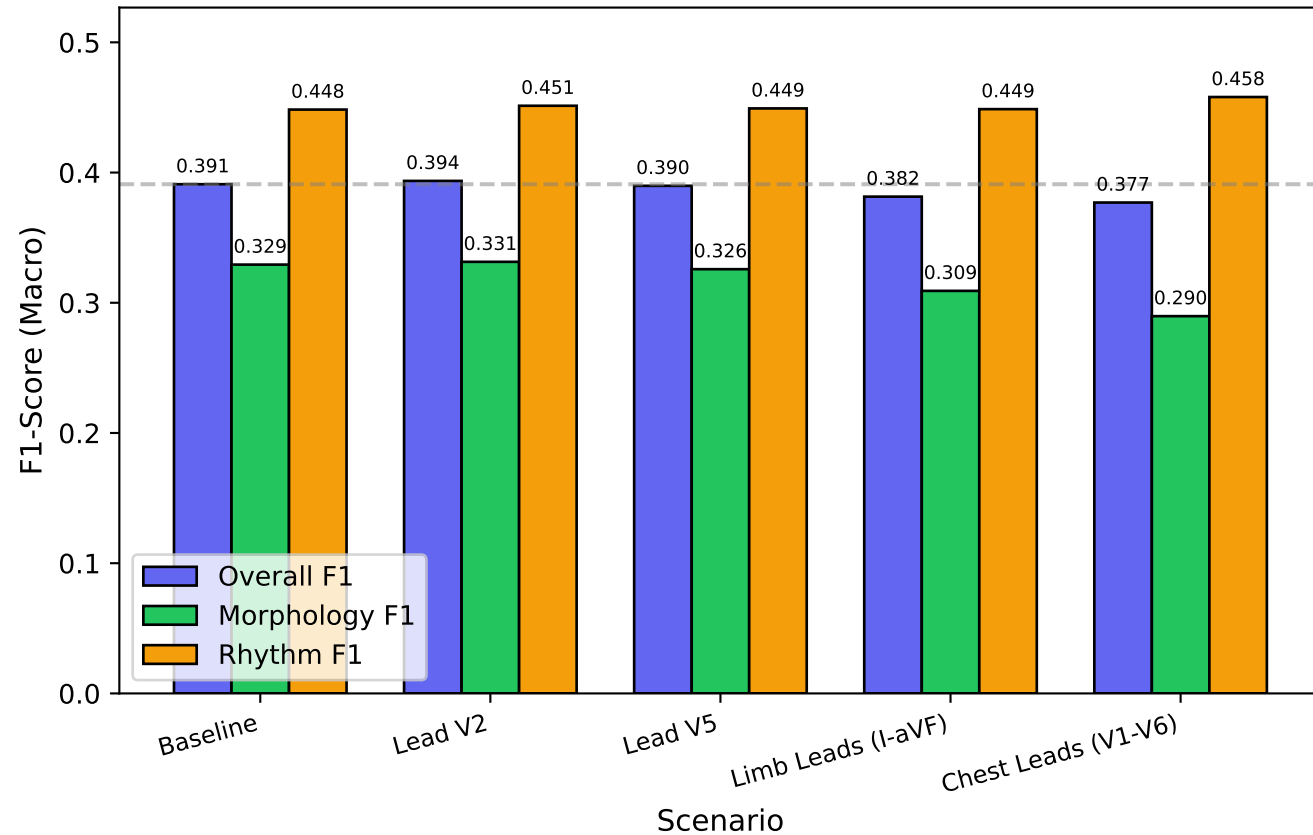
Lead Dropout: F1 by Class Group
