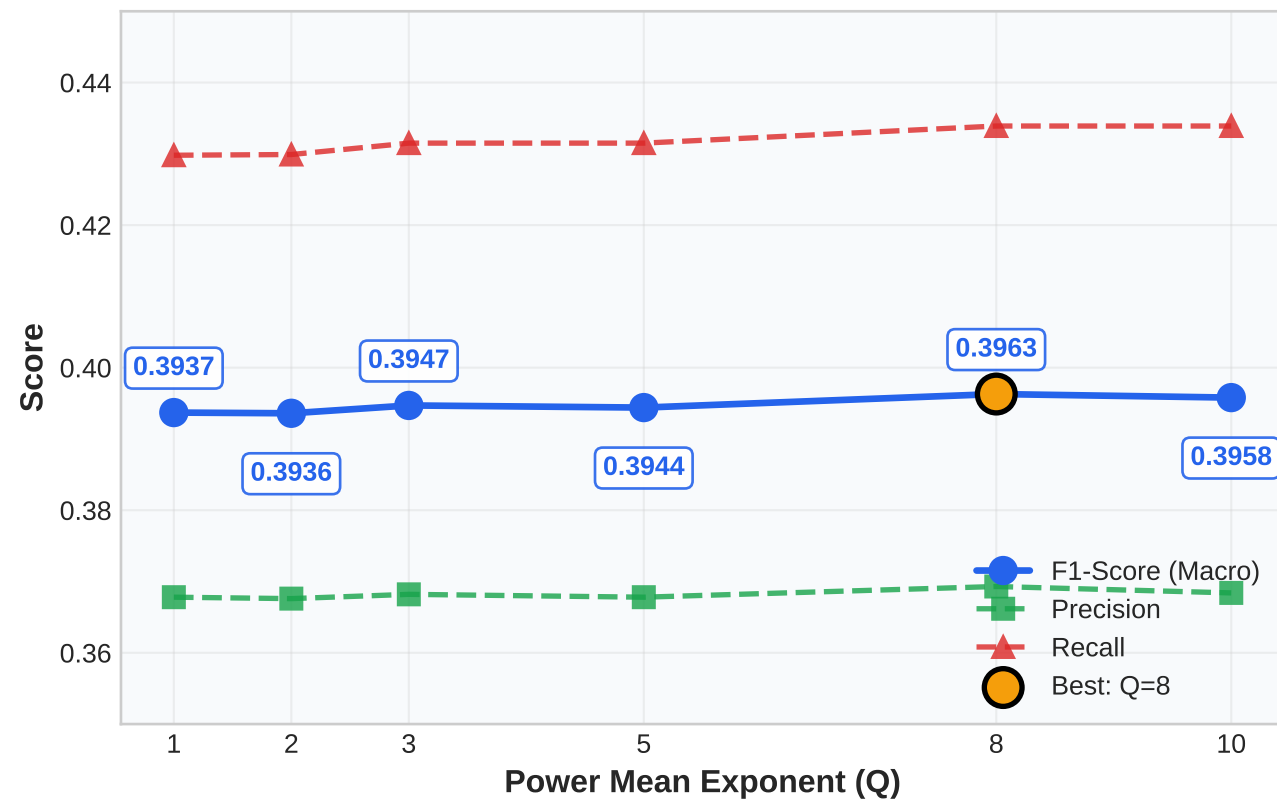
(a) Sensitivity Analysis: F1 vs Q
