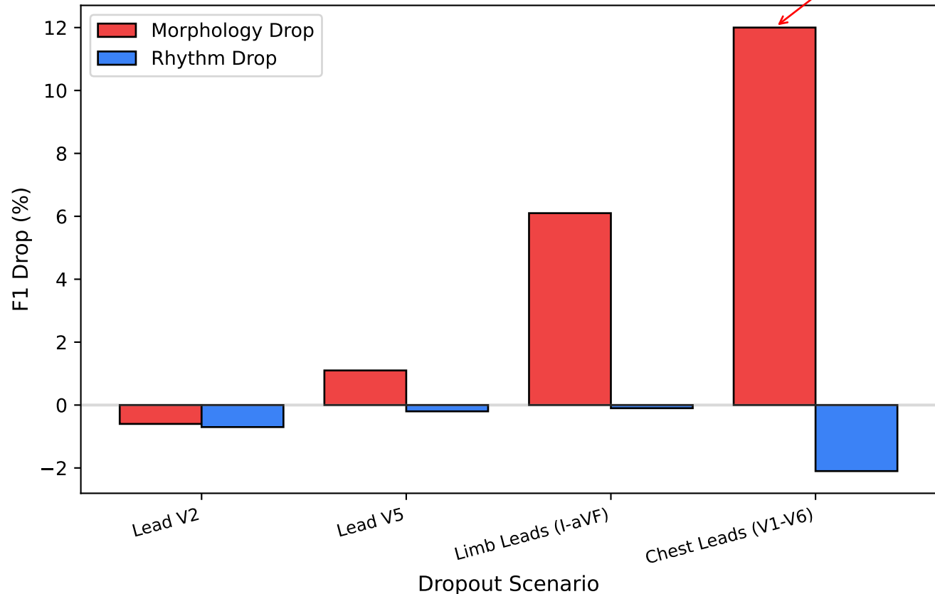
Spatial Dependency: Morphology vs Rhythm
