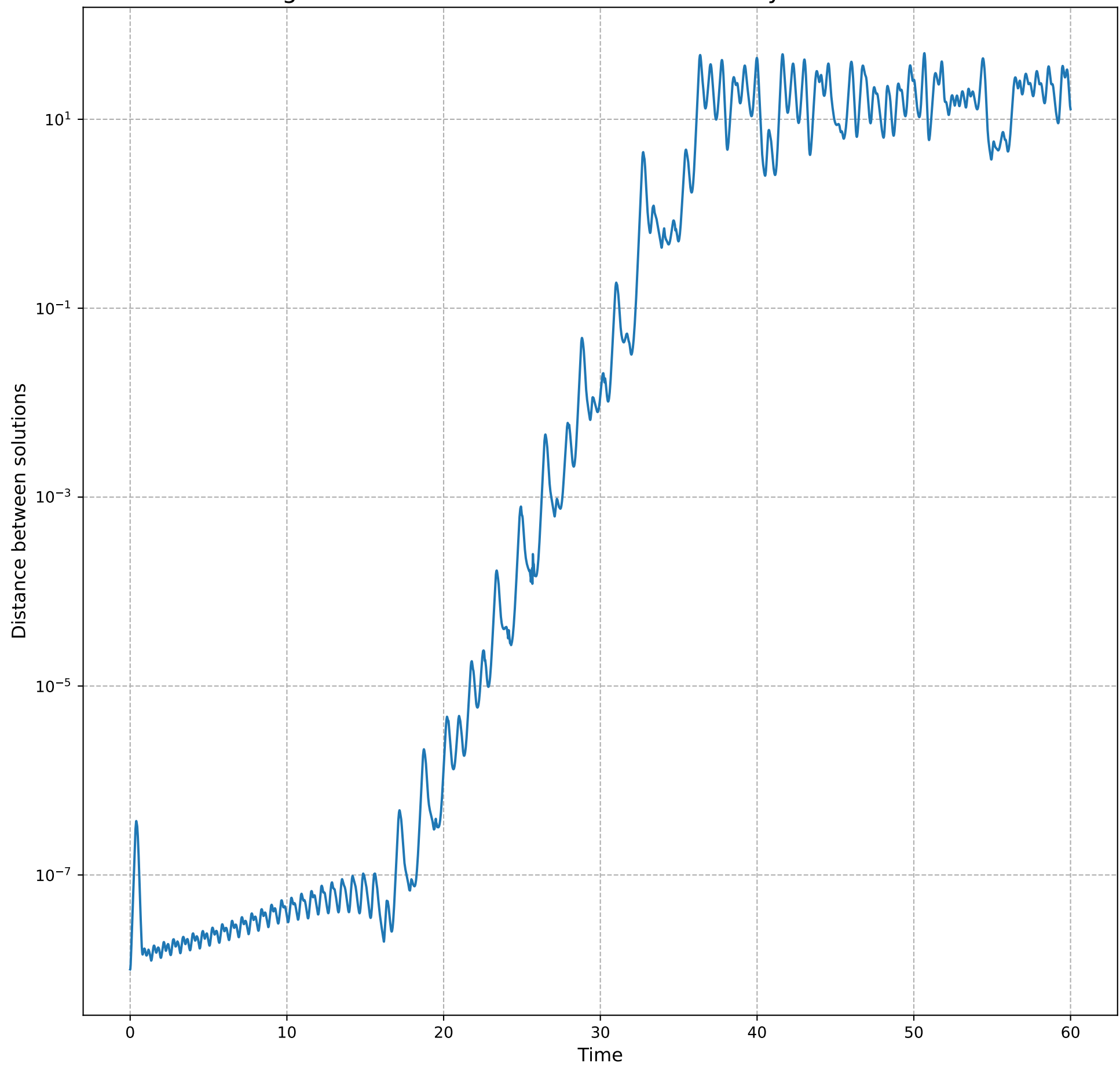
Divergence After a Small Perturbation Nearby Initial Condition
