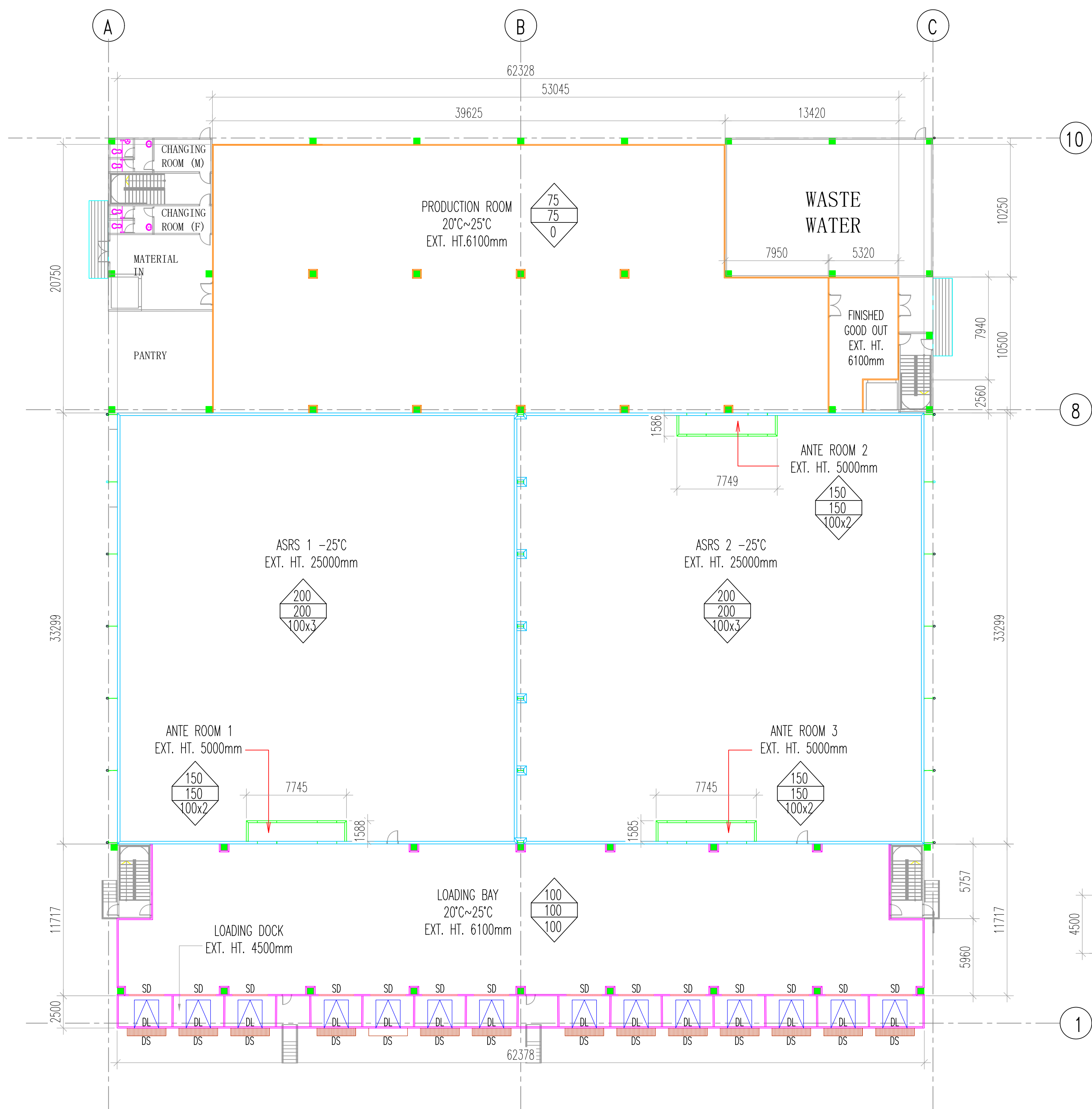
WALL LAYOUT PLAN
