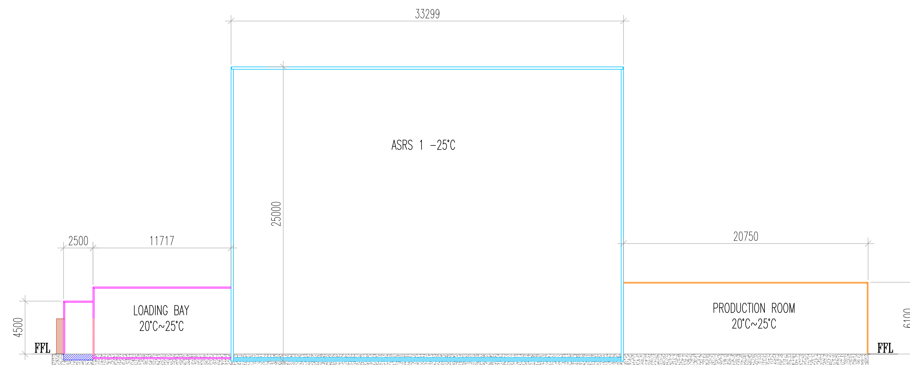
SIDE ELEVATION
