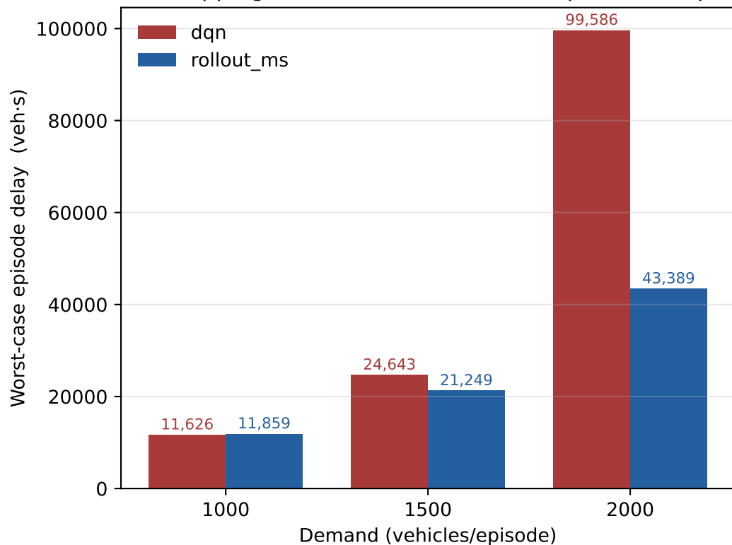
Tail clipping: rollout truncates catastrophic blow-ups
