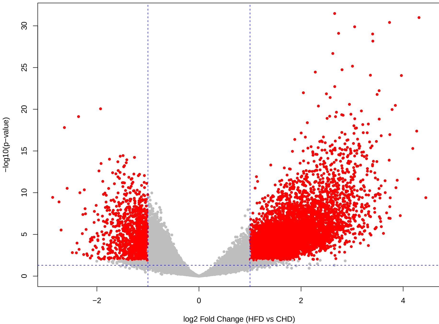
Volcano: HFD vs CHD
