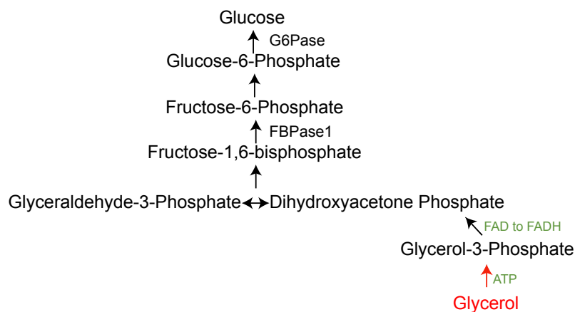
Figure 36: Schematic of gluconeogenesis from glycerol. Red indicates key gluconeogenic substrates while green indicates energy consuming or generating steps. Based on this diagram, you can see that per glycerol 1 ATP is used, and 1 FADH 2 is generated. This is a net of +0.5 ATP/glycerol, or since two glycerol molecules are needed to make a glucose, a net ATP increase of 1 ATP/glucose generated.
