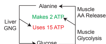
Figure 40: Schematic of the Cahill Cycle. Each turn through this cycle uses up 13 ATP (15 ATP used in the liver, 2 generated in the muscle).
