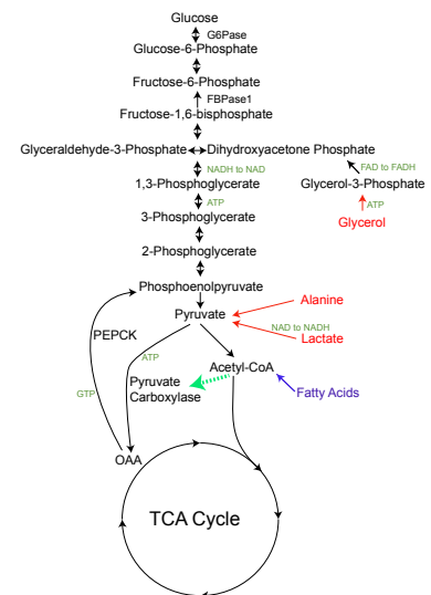
Figure 35: Schematic of gluconeogenesis. Red indicates key gluconeogenic substrates while green indicates energy consuming or generating steps.
