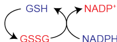
Figure 27: The glutathione:NADPH antioxidant system. The oxidized form of each molecule is shown in orange, the reduced form is in blue.
