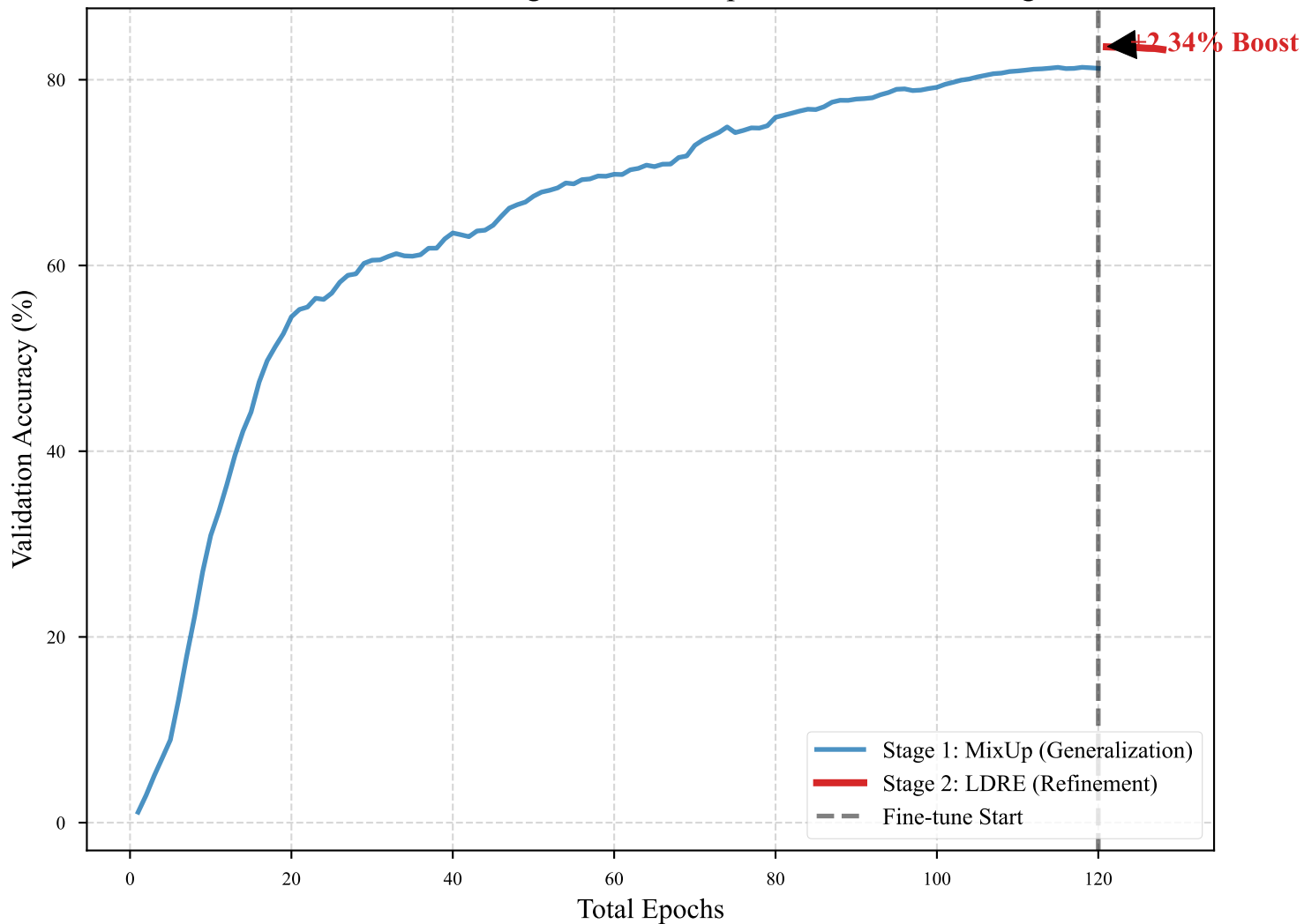
Curriculum Learning Effect: MixUp -> LDRE Fine-tuning
