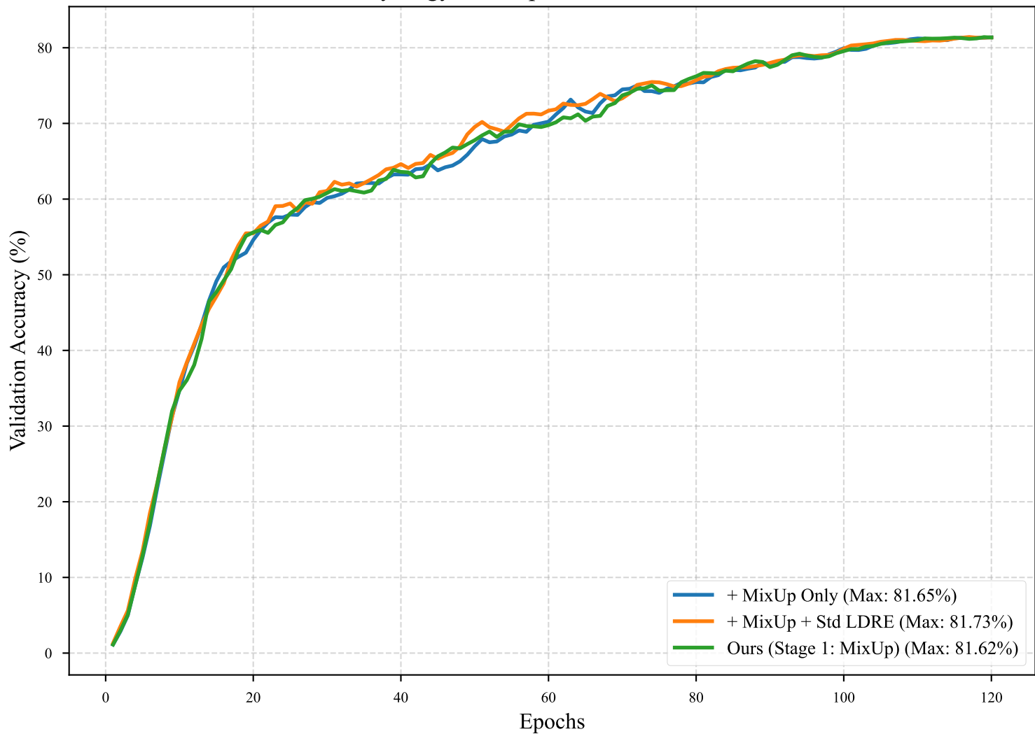
Synergy: MixUp vs LDRE Variants
