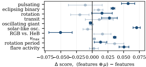
(a) gain over engineered features
