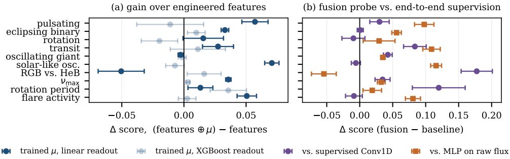
Figure 1: The two claims. (a) What the learned features add to the engineered features, under the fixed linear readout of Table 1 (solid) and under an XGBoost readout on the same inputs (faded; Appendix B). (b) The fusion probe against the two supervised baselines. Bars are 2 SE.
