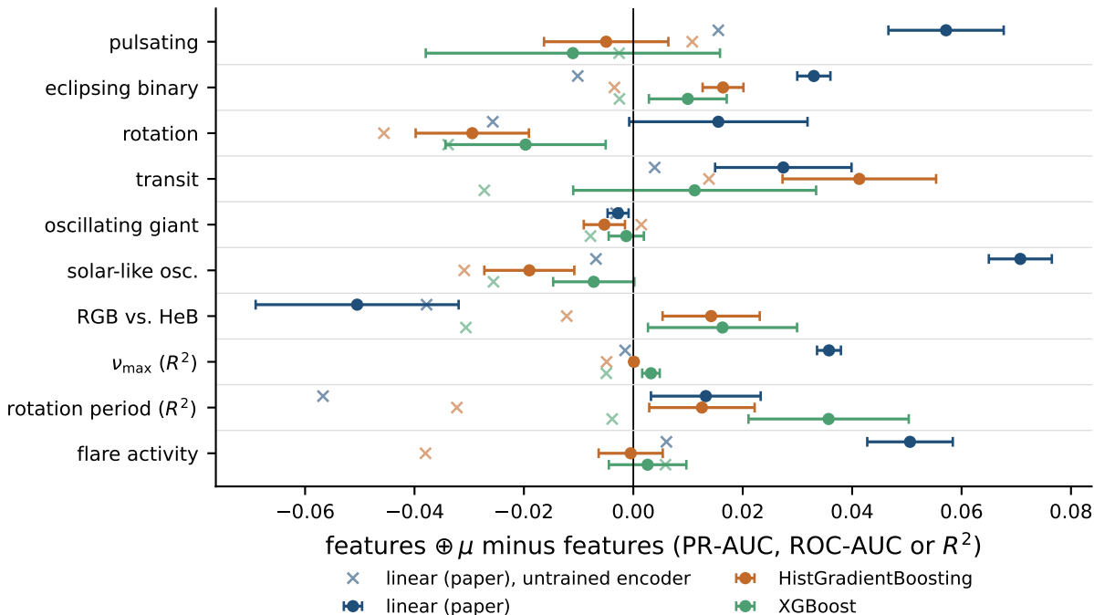
Fusion gain under three readouts on the same feature sets; bars are 2 SE over six seeds, x marks the untrained-encoder control
