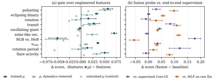
Figure 1: The two claims. (a) What the learned features add to the engineered features under the same fixed linear readout, for the shipped encoder, its dynamics-free twin and an untrained control. (b) The fusion probe against the two supervised baselines. Bars are 2 SE; the untrained control is a single encoder and carries none.
