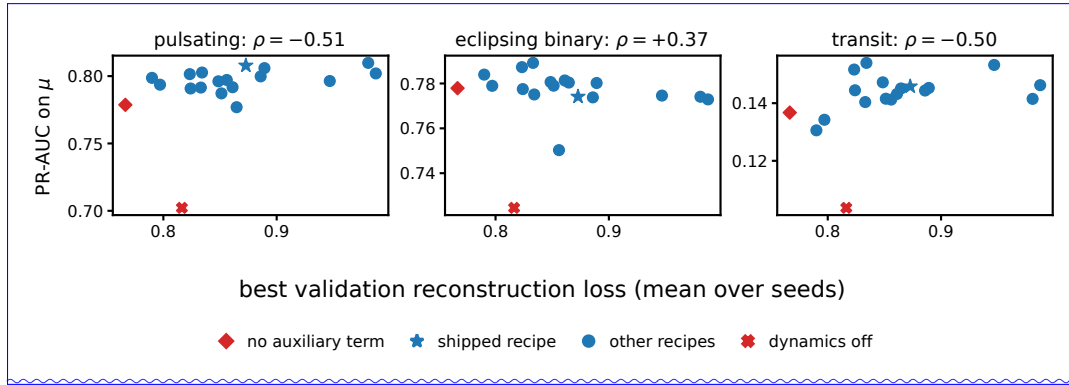
Figure 3: The same estimator as Figure 2, on the family our encoder belongs to: 19 recipes on the final encoder that vary the form, weight and floor of the spectral auxiliary term, six seeds each. The diamond has no auxiliary term, the cross is the one dynamics-off recipe, the star is the recipe we use. x : best post-warm-up validation reconstruction loss; y : PR-AUC of the fixed linear probe on \mu ; \rho : Spearman’s rank correlation between negated loss and score.
