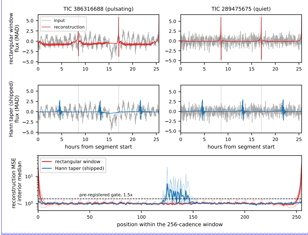
Figure 4: The artifact, in two stars and in the average. Top two rows: three consecutive 256-cadence windows of one pulsator and one quiet star, input flux in grey against each recipe’s reconstruction; dotted lines mark the window boundaries, and both rows of a column share one y -scale. The two recipes differ only in the taper used for the auxiliary spectral term. Neither decoder reproduces the cadence-scale scatter, which a 128-dimensional bottleneck cannot carry; what differs is where each one puts a spike it does not need. Bottom: reconstruction error by position within the window, divided by that seed’s median over positions 16–240. Thin lines are the six pre-training seeds, thick lines their mean. The dashed line is the pre-registered artifact gate. The seed mean understates the tapered recipe’s peak because its position moves between seeds (125–143), which is why the gate is read as a maximum within each seed.
