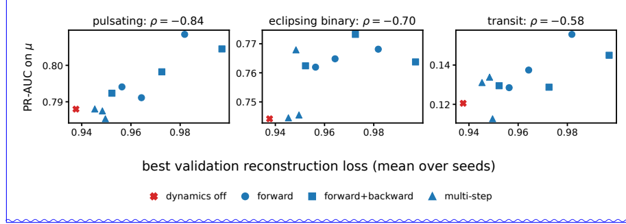
Figure 2: Validation reconstruction loss against downstream probe score, one point per pre-training recipe and one panel per task; the rotation tasks are absent because these recipes were never encoded on the pool rotation is scored on. The ten recipes share corpus, architecture and loss terms and differ only in the GRU prediction term (off, forward, forward+backward, multi-step, the last three at three weights), four seeds each. x : best post-warm-up validation reconstruction loss, averaged over the recipe’s seeds; y : PR-AUC of the fixed linear probe on \mu ; \rho : Spearman’s rank correlation between negated loss and score. The loss-optimal recipe is the dynamics-free one (red) on all three tasks, and it is the worst or next-to-worst probe on each. Appendix E repeats the measurement on the family this paper’s encoder belongs to.
