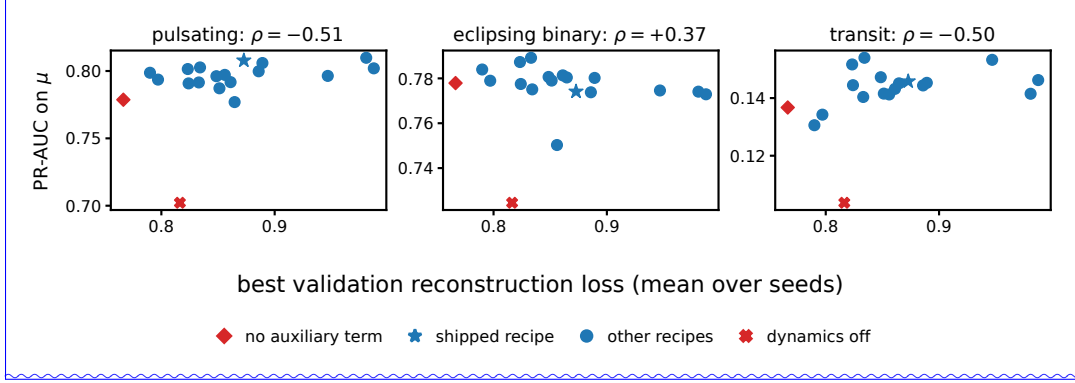
Figure 3: The same estimator as Figure 2, on the 19 variants of our final recipe. The diamond has no auxiliary term, the cross is the one variant without the GRU prediction term, the star is the recipe we use. x : best post-warm-up validation reconstruction loss; y : PR-AUC of the fixed linear probe on \mu ; \rho : Spearman’s rank correlation between negated loss and score.
