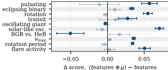
(a) gain over engineered features
