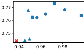
eclipsing binary: \rho = -0.70
