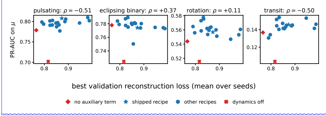
Figure 3: The same estimator as Figure 2, on the family our encoder belongs to: 19 recipes on the final encoder that vary the form, weight and floor of the spectral auxiliary term, six seeds each. The diamond has no auxiliary term, the cross is the one dynamics-off recipe, the star is the recipe we use. x : best post-warm-up validation reconstruction loss; \mu : PR-AUC of the fixed linear probe on \mu ; \rho : Spearman’s rank correlation between negated loss and score.
