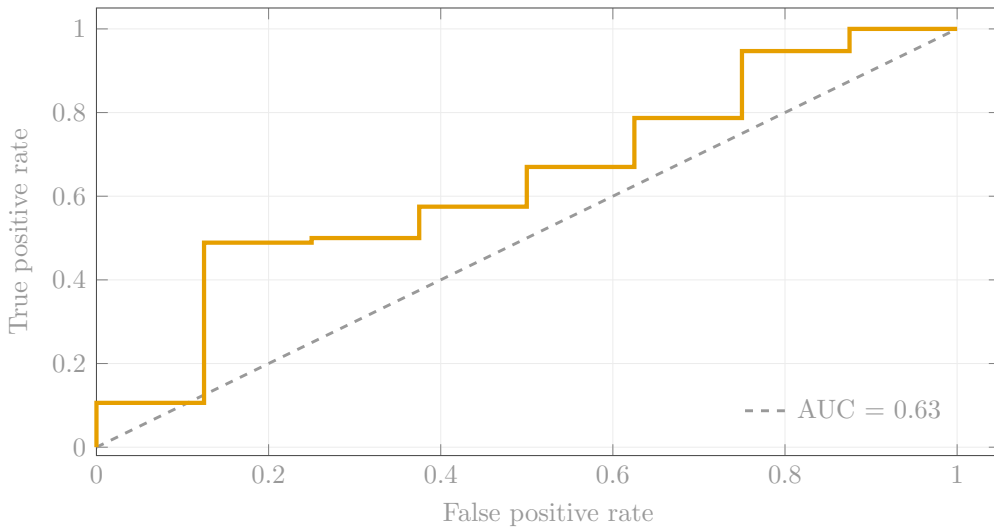
Figure 5: ROC curve for the turn-aware confidence estimator ( AUC = 0.634 ). The dashed diagonal represents the random baseline ( AUC = 0.500 ). N = 102 labeled turns (94 correct, 8 incorrect).
