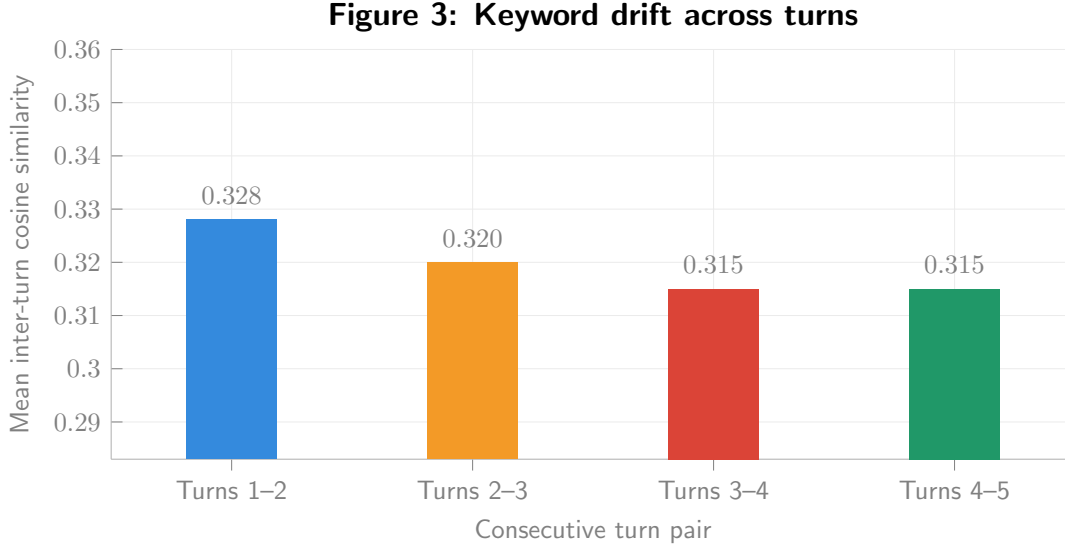
Figure 3: Inter-turn keyword similarity declines as reasoning progresses, indicating semantic drift from the original query topic (0.328 \rightarrow 0.315 from turns 1-2 to turns 3-4).
