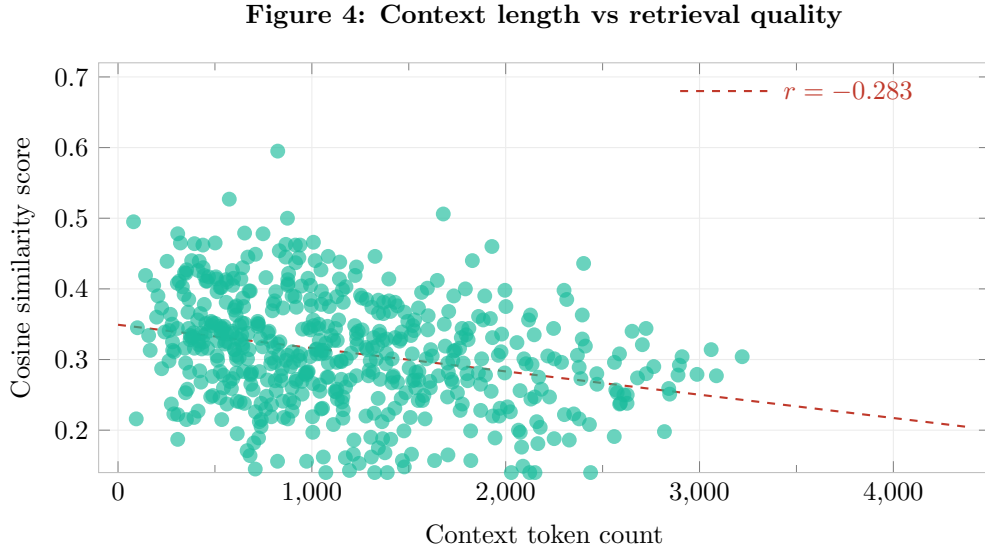
Figure 4: Strong negative correlation between context token count and retrieval cosine similarity (Pearson r = -0.283 , p < 0.0001 , n = 547 Tier 1 turns). Each dot represents one logged reasoning turn. Dashed line = linear regression.
