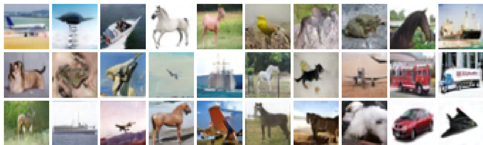
Gaussian (fKL)
