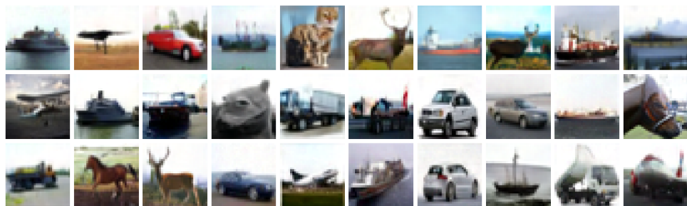
Gaussian (rKL)
