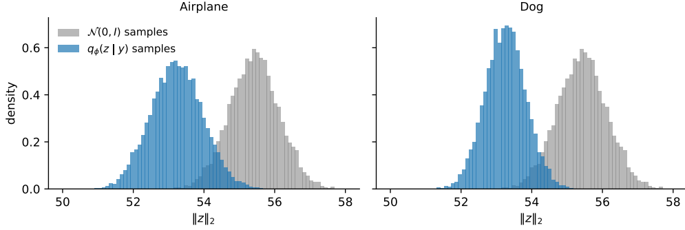
Figure 5.11: Norms of 10,000 latents produced by the noise adapter for each of the two observations of Figure ??, against 10,000 standard-normal samples. For z \sim \mathcal{N}(0, I_D) with D = 3072 , \|z\|_2 follows a chi distribution with mean \sqrt{D-1}/2 \approx 55.4 and standard deviation 1/\sqrt{2} \approx 0.71 .
