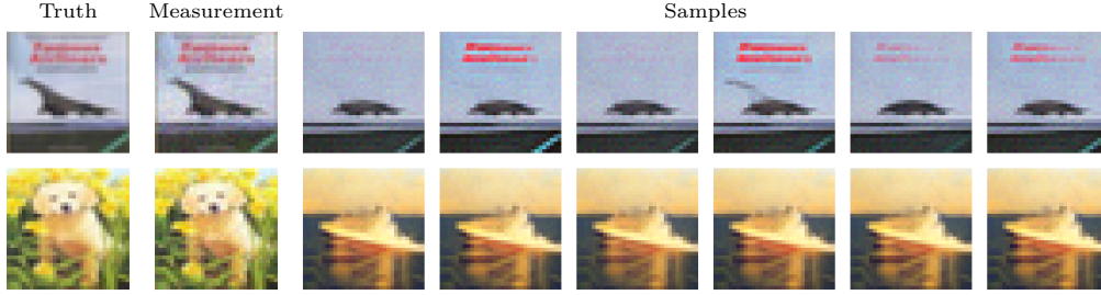
Figure 5.13: Inversion: the same two images as Figure ?? (top: airplane, bottom: dog), now observed in full with measurement noise ( \sigma = 0.05 ), and six samples from an adapter trained for this inversion task. Even with every pixel observed, the adapter does not recover the image; for the dog it produces a ship.
