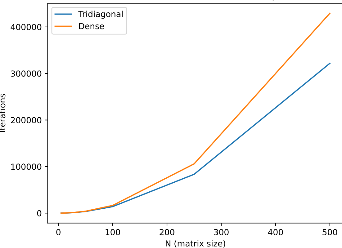
Iterations needed as function of size, tridiagonal matrix
